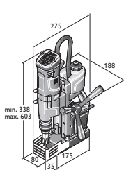
KBU 35 Q KBU 35 QW
